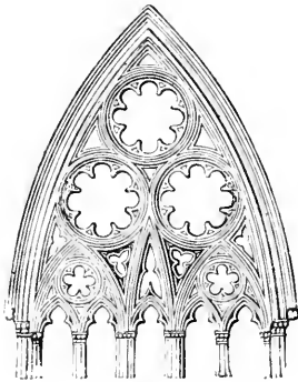
Fig. 238. Decorated window.
